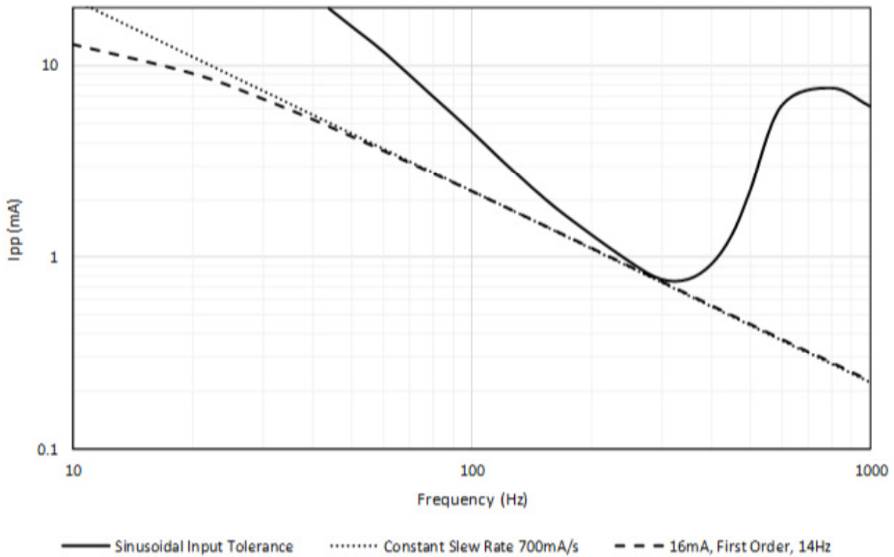
Figure 32 - Analogue Input Slew Tolerance
